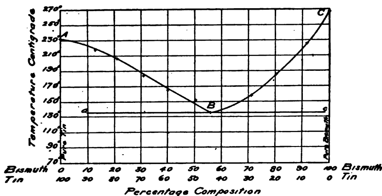
Fig. 33. Freezing-point Curve of the Bismuth-tin Alloys.
